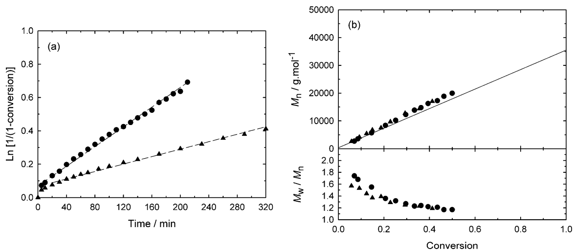
Figure 5. Bulk copolymerization of methyl methacrylate and styrene (initial molar fraction of styrene: f_{S0} = 0.088 ) at 83 ( P4 , ●) and 78 °C ( P5 , ▲), in the presence of 2.66 \times 10^{-2} \text{ mol L}^{-1} of MAMA ( M_{n(x=1)} = 35\,520 \text{ g mol}^{-1} ), 10.3 mol % of added free SG1 based on the initiator. Key: (a) \ln[1/(1-x)] vs time ( x = overall conversion); (b) number-average molar mass, M_n , and polydispersity index, PDI, vs conversion. The full line represents the theoretical M_n .
